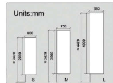
Indoor Flag Pole Dimensions
